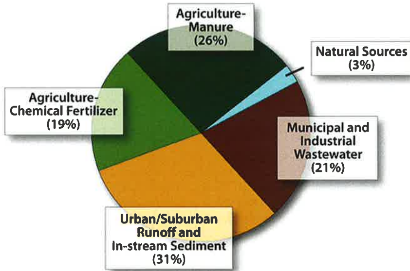
FIGURE 1-7 Sources of phosphorus to the Chesapeake Bay.
