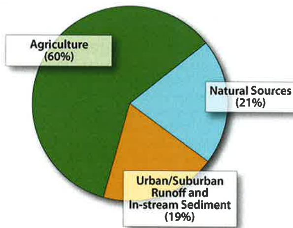
FIGURE 1-8 Sources of sediment to the Chesapeake Bay.
