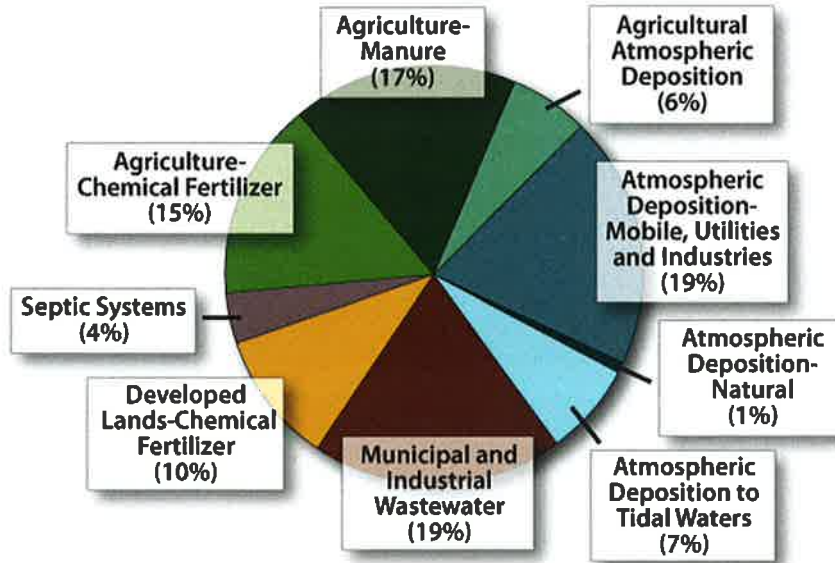
FIGURE 1-4 Sources of nitrogen to Chesapeake Bay.
