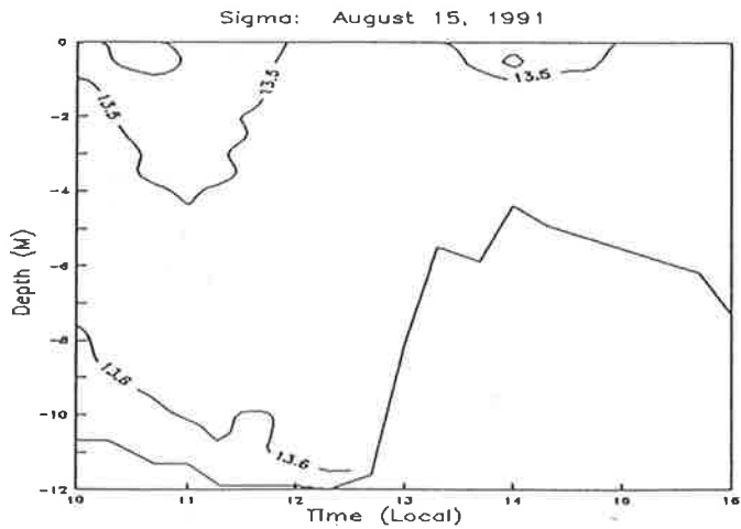
IV-1-2 Vertical structure of temperature, salinity, and density ( \sigma ) [top to bottom] as functions of time along the drogue trajectory.
