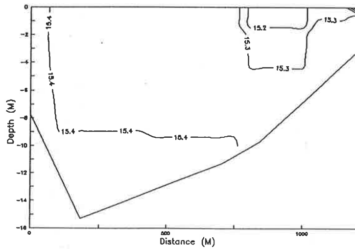
Sigma: October 3, 1991 (B)
