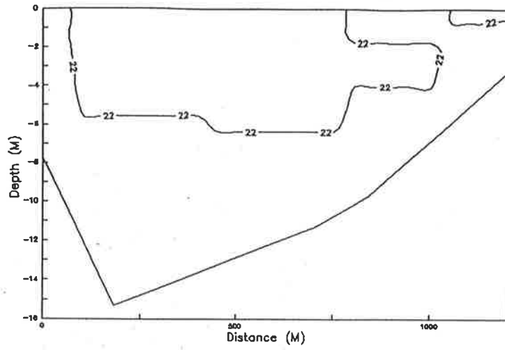
Water Temperature: October 3, 1991 (B)
