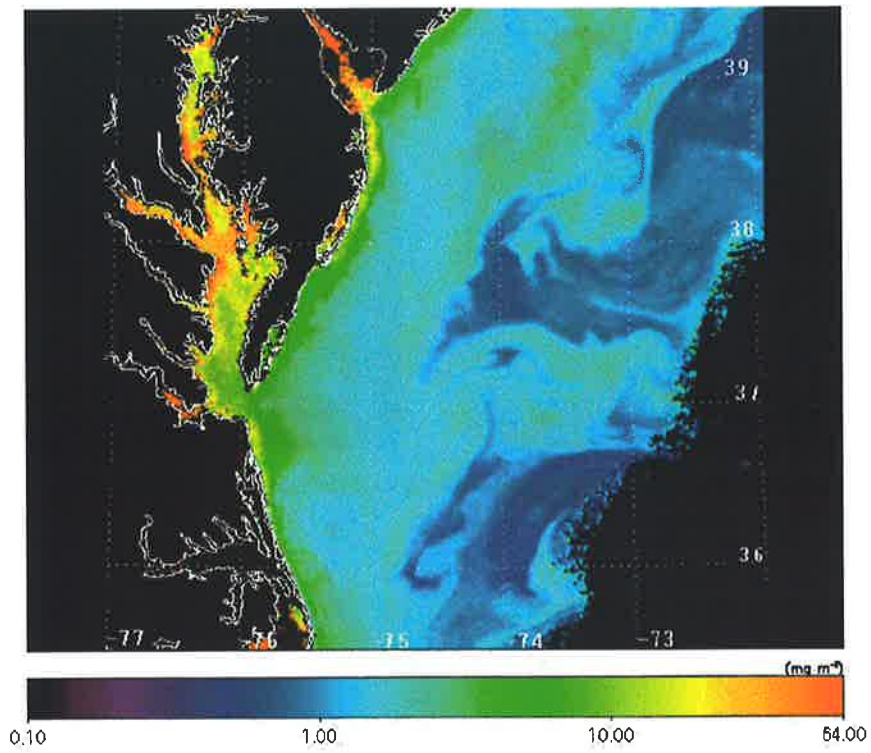
SeaWiFS K490 ( \text{m}^{-1} ) on April 12, 1998
