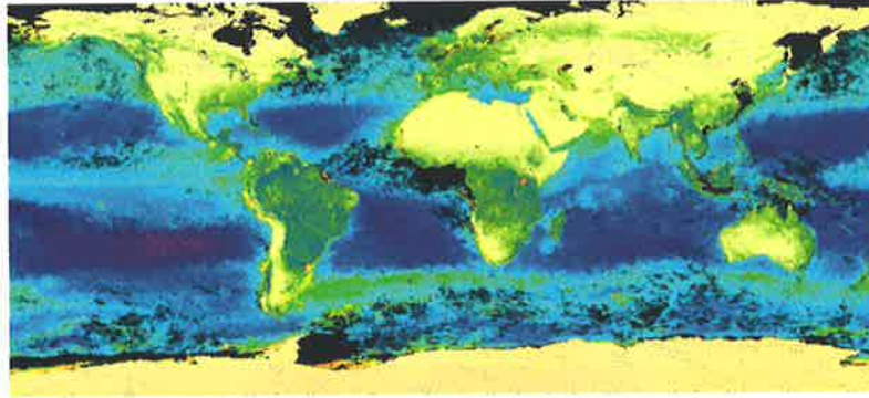
Figure 1. Global chlorophyll (chl-a) in the terrestrial and ocean biosphere from SeaWiFS.
