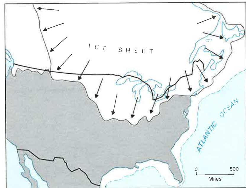
Figure 3. Maximum extent of ice 18,000 years ago during the last glaciation. Sea level was over 300 feet below its present level, and the shoreline at that time was hundreds of miles offshore (see dashed line).
