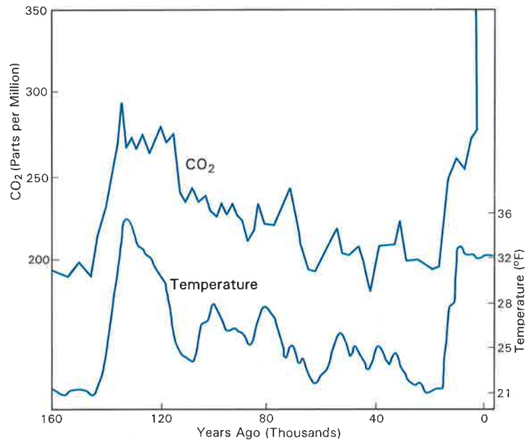
Figure 7. Correlation between temperature change and an increase of atmospheric \text{CO}_2 (Intergovernmental Panel on Climate Change, 1990).
