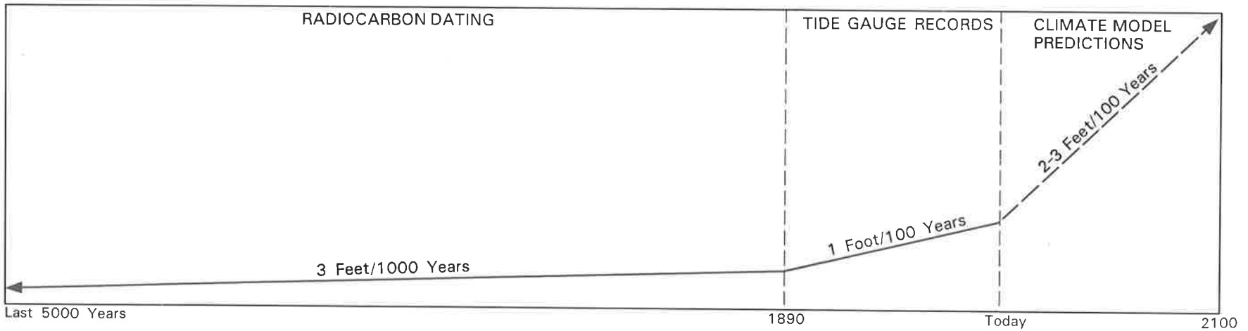
Figure 10. Sea-level rise curve: past and projected.
