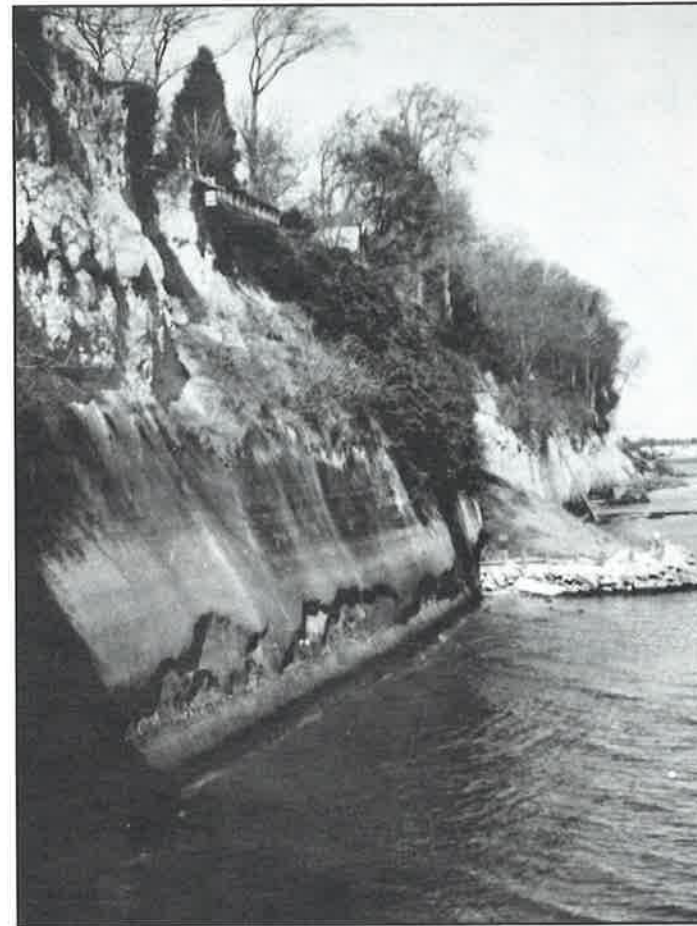
Figure 11. Much of the Western Shore of Chesapeake Bay is characterized by erosional cliffs (photo by Stephen Leatherman).
