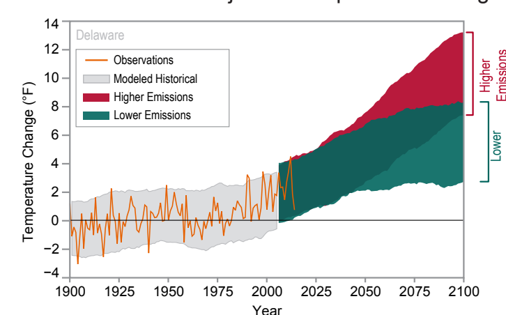
Figure 1: Observed and projected changes (compared to the 1901–1960 average) in near-surface air temperature for Delaware. Observed data are for 1900–2014. Projected changes for 2006–2100 are from global climate models for two possible futures: one in which greenhouse gas emissions continue to increase (higher emissions) and another in which greenhouse gas emissions increase at a slower rate (lower emissions). 1 Temperatures in Delaware (orange line) have risen more than 2°F since the beginning of the 20th century. Shading indicate the range of annual temperatures from the set of models. Observed temperatures are generally within the envelope of model simulations of the historical period (gray shading). Historically unprecedented warming is projected during the 21st century. Less warming is expected under a lower emissions future (the coldest years being about 3°F warmer than the long-term historical average; green shading) and more warming under a higher emissions future (the hottest years being about 13°F warmer than long-term historical average; red shading). Source: CICS-NC and NOAA NCEI.
