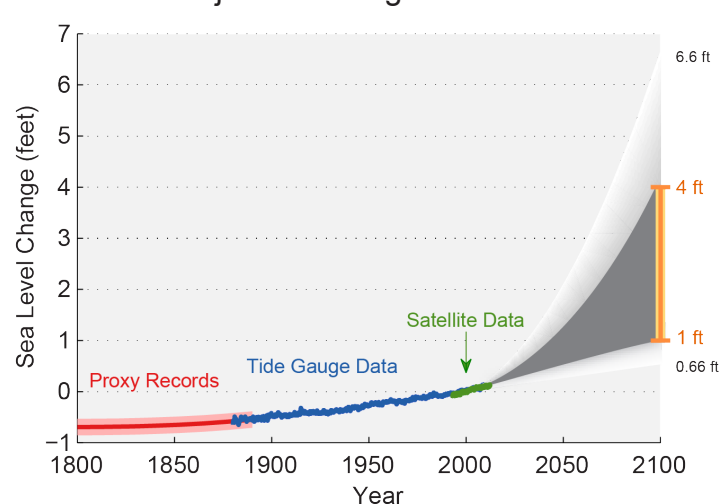
Figure 6: Estimated, observed, and possible future amounts of global sea level rise from 1800 to 2100, relative to the year 2000. The orange line at right shows the most likely range from climate models of 1 to 4 feet by 2100 based on an assessment of scientific studies, which falls within a larger possible range of 0.66 feet to 6.6 feet. Source: Melillo et al. 2014 and Parris et al. 2012.
